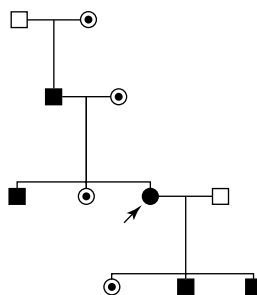
Figure 2.23 Occurrence of an affected homozygous female in a common X-linked recessive trait, red-green colour-blindness.
